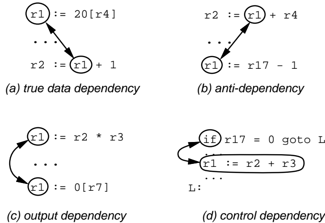
Figure 3: Dependencies
